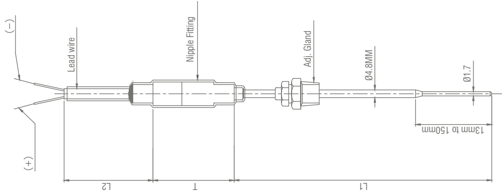
Swaged Type Special Thermocouple Assembly for Quick Response
