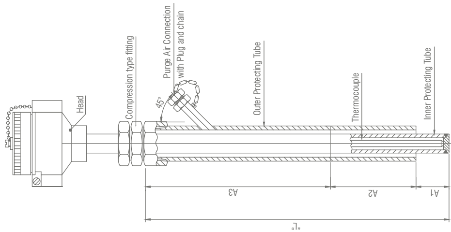
BED Type Thermocouple Assembly
