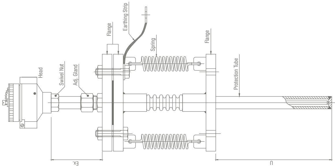
Fully Spring Loaded Thermocouple / RTD Assembly for Vibration Application
